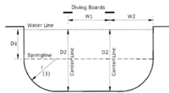
Transverse Section Deep End
