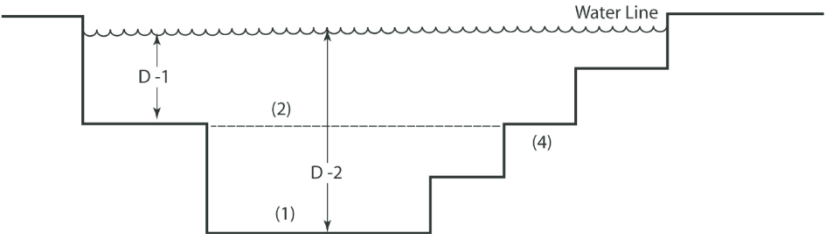
Figure 31B-6 Depths and Dimensions for Spa Pools
