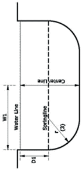
Figure 31B-3 Depths and Clearances for Pools without Diving Boards
